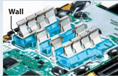
Terminal short-circuit prevention structure
